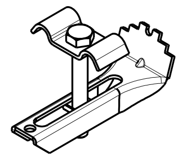
scale 1:2 ISO-view
